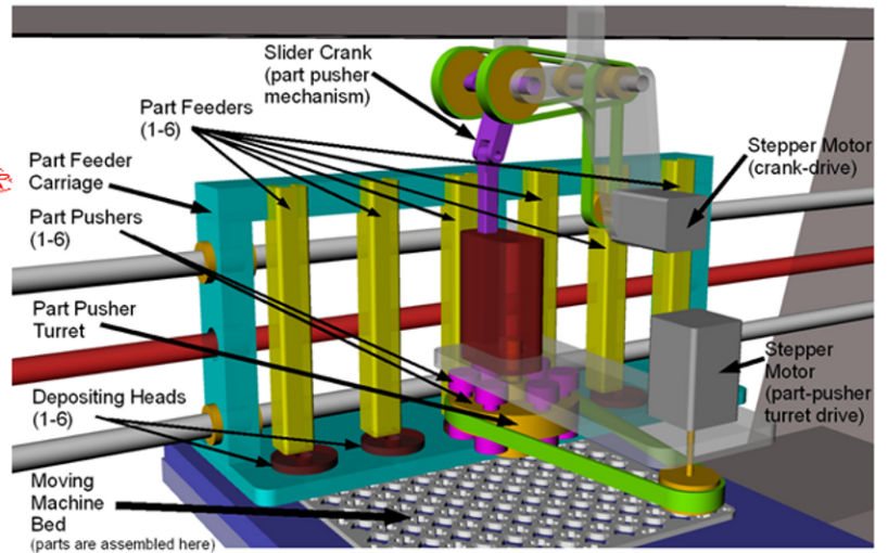
Voxel Assembling Head
