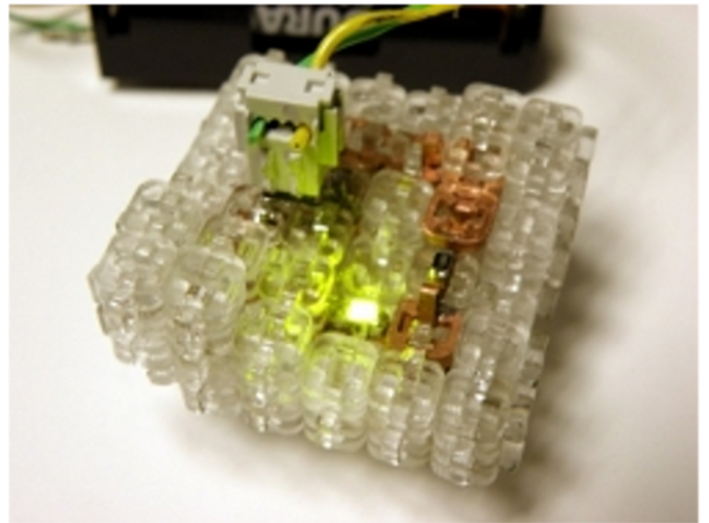
Voxel Assembling Head
