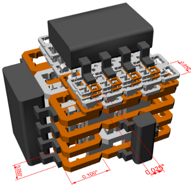
Voxel Assembling Head
