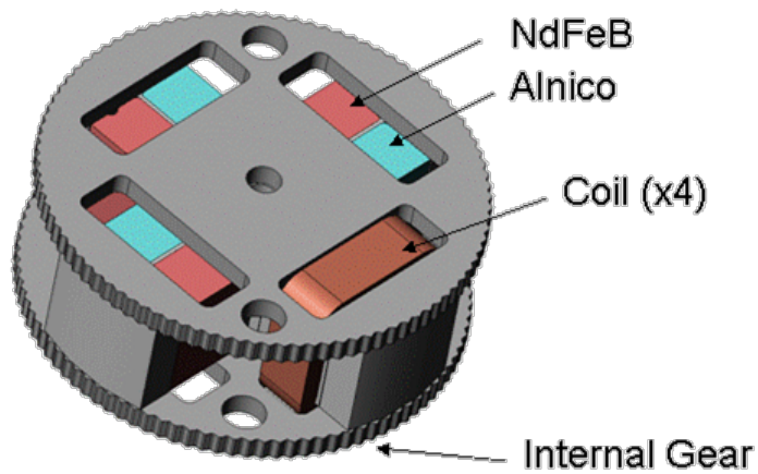
Electropermanent Wobble Stepper Motor with Continuous Gearing
