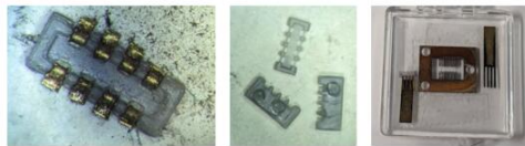
Figure 5.1: Connectors fabricated using a combination of desktop fabrication tools
