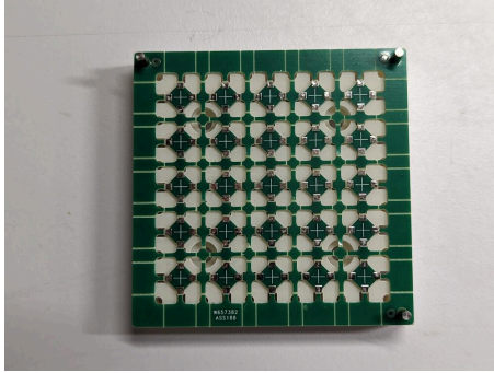
(a) dowels
