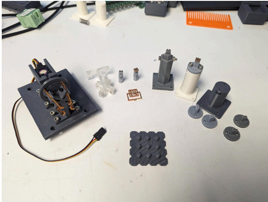
Figure 3.10: Passive gripper end effector for 4Hp H-eon connector
