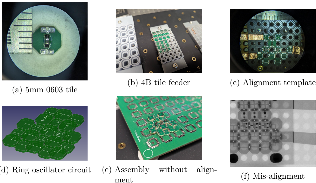
Figure 2.12: 4B design and assembly tests
