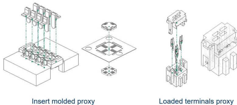
Figure 5.2: Assembly techniques
