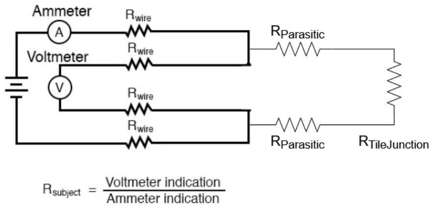
Figure 4.7: 4-wire test setup, measuring R_{PadJunction}
