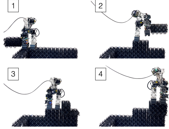
Figure 13: A single robot assembling a support staircase for the bench build.
